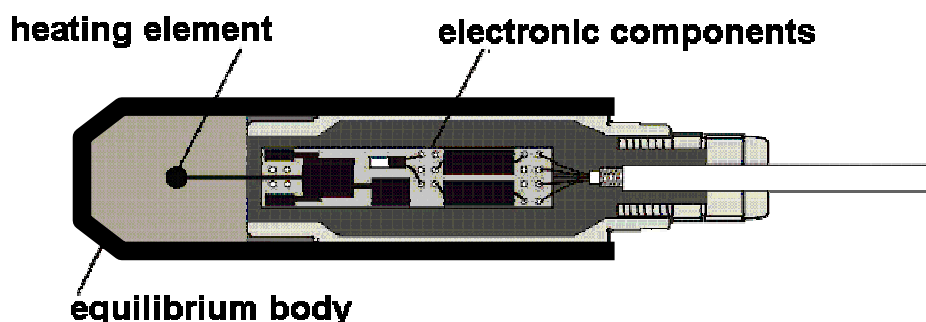
Fig. 2: Structure of the Tensiomark
