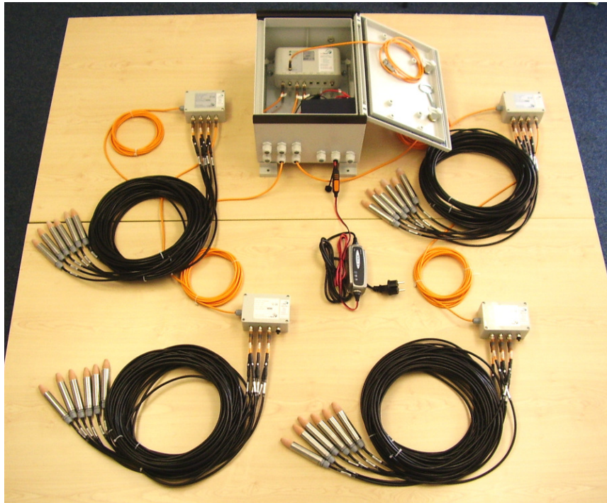
Fig. 5: Measuring system, consisting of a data logger enviLog Maxi, 4 SDI-12-multiple sockets and 24 pF-Meters
