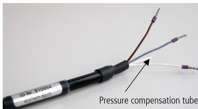
Fig. 8: Wire assignment of a Tensiomark in the analog mode
