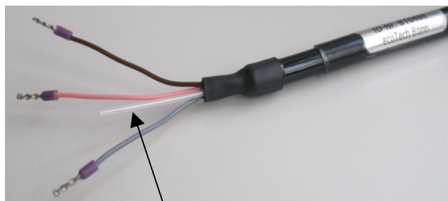
Pressure compensation tube
